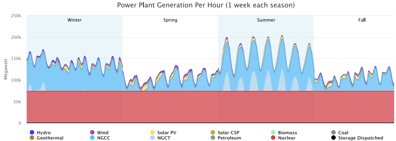
Figure 2. (with electricity storage) Hourly dispatch by type of electricity generation.
